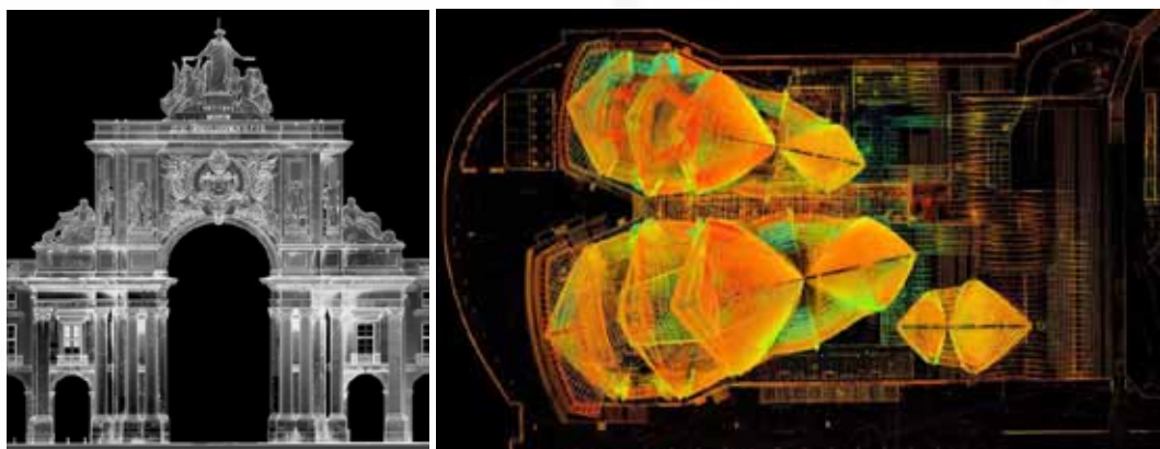
Figure 27. The 3D laser scanning survey of the Arco of Rua Augusta. Figure 28. The Sydney Opera House project took more than 800 laser scans of the interior and exterior, and 56,000 digital photos, documenting 13 billion measurable points on the structure using cutting-edge, laser-mapping technologies (“3D laser scanning,” 2013).
