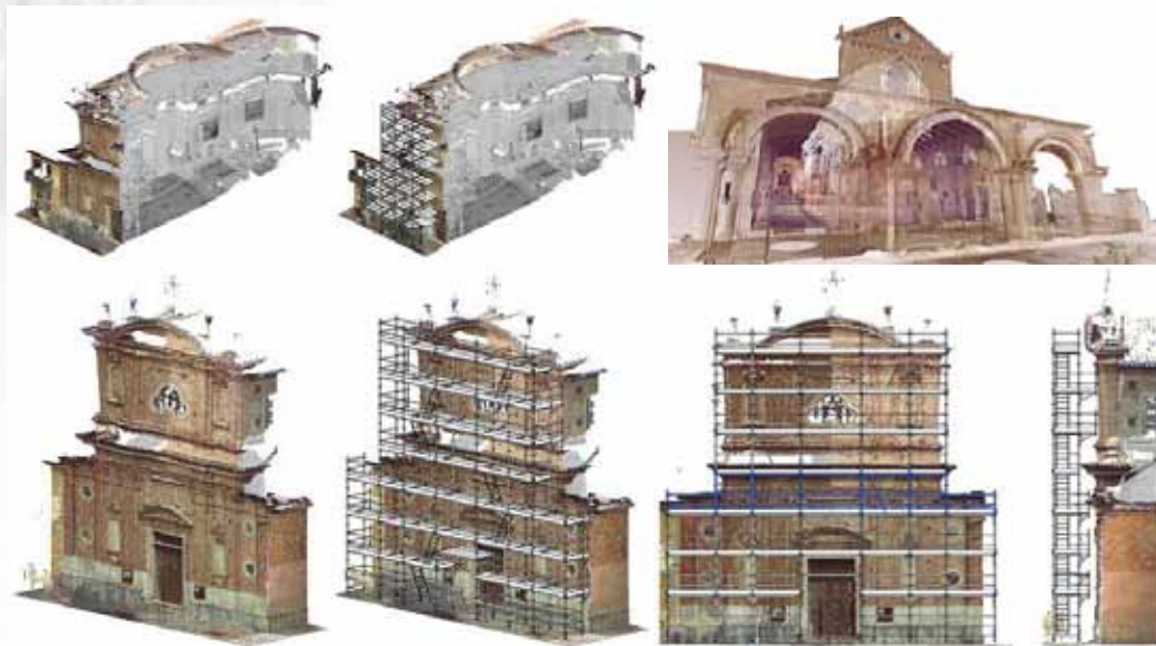
Figure 30. Digital photogrammetry and laser scanning (“Digital photogrammetry and laser scanning,” 2018) (“3d scanning,” 2018).
