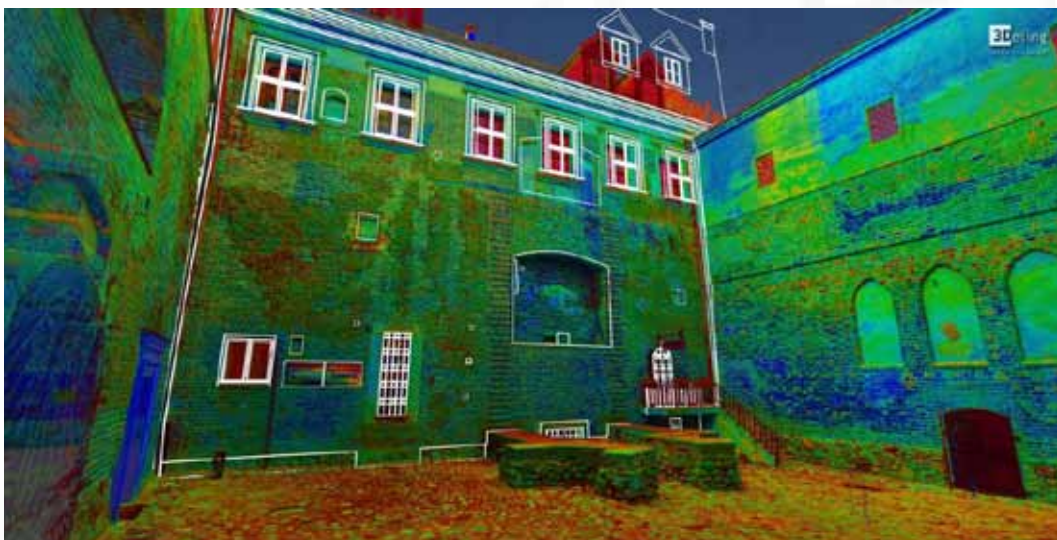
Figure 53. The building was scanned at the highest resolution settings for all external interfaces. Then, it was covered by the CAD with Orthoimages to show the full potential of laser scanning (“3Ddeling - 3D Laser scanning,” 2018).
